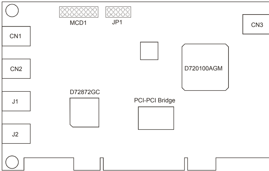
Fig. 1.1 Key Components of PTI-213C
