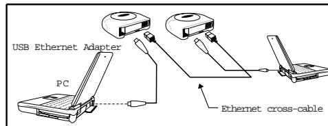
Figure 2-2: PC-to-PC Direct Connections
